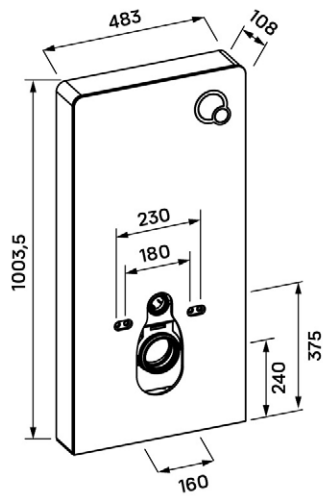
CORSICA + CORSICA BLACK TOILET TANK OUTSIDE THE WALL FOR WALL-MOUNTED TOILETS
