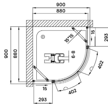
SCORPIO SHOWER CABIN
