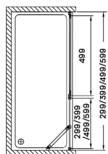
PURE 90/100/110/120 SHOWER WALL
