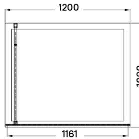
TINO WALK-IN SHOWER WALL
