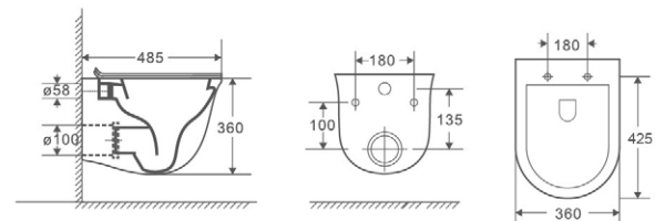
OLIVIA WALL-MOUNTED RIMLESS TOILET
