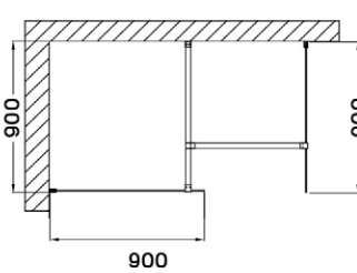
ASTRO 140 WALK-IN SHOWER WALL
