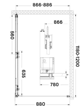
FABIO SHOWER CABIN
