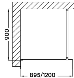
ASTRO CORNER 90/120 WALK-IN SHOWER WALL
