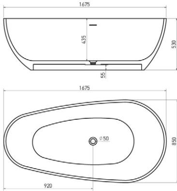
SOUL MATT WHITE + MATT BLACK FREESTANDING CAST MARBLE TUB
