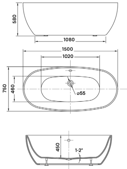
ALASSIO FREESTANDING BATHTUB
