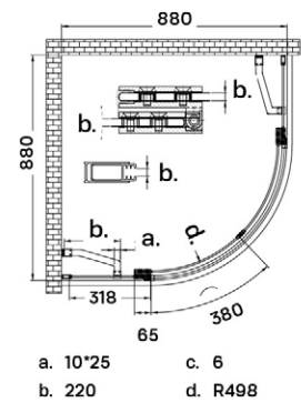
ARNO SHOWER CABIN
