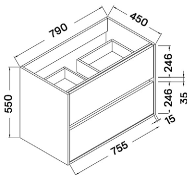
ALMERIA 80 BASIN CABINET
