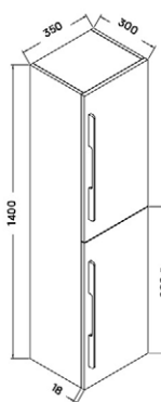
NINA SUSPENDED TALL CABINET
