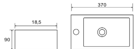
VIOLET WALL-MOUNTED PORCELAIN BASIN
