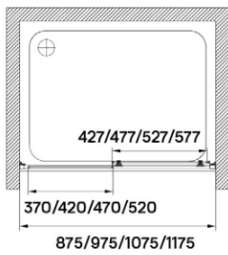
PREMIER 90/100/110/120 SHOWER WALL
