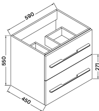
NINA 60 BASIN CABINET
