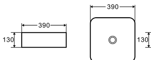
AZALEA MATT / AZALEA B&W COUNTER-TOP PORCELAIN BASIN
