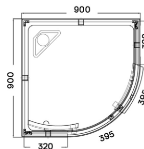
VIVARA SHOWER CABIN WITH BACK WALL AND TRAY
