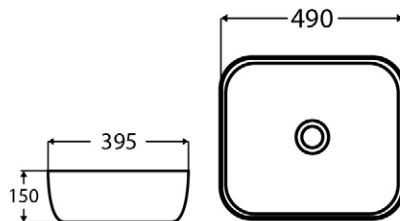
DAISY COUNTER-TOP PORCELAIN BASIN
