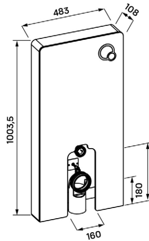
CORSICA + CORSICA BLACK TOILET TANK OUTSIDE THE WALL FOR FLOOR-STANDING
