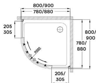
AQUARIUS 80/90 SHOWER CABIN
