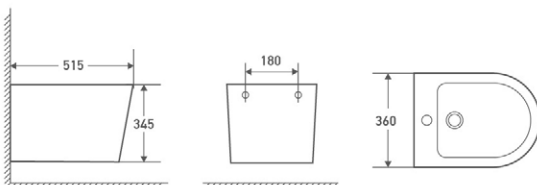
CLEMENT + CLEMENT BLACK WALL-MOUNTED BIDET
