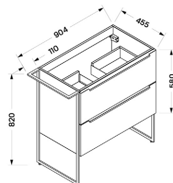
JERSEY BASIN CABINET
