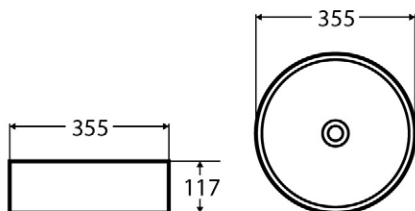
ROSE / ROSE MATT / ROSE BLACK / ROSE B&W COUNTER-TOP PORCELAIN BASIN
