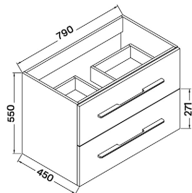
NINA 80 BASIN CABINET
