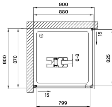
QUADRUN + QUADRUN BLACK SHOWER CABIN
