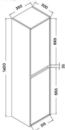
GINGER SUSPENDED TALL CABINET
