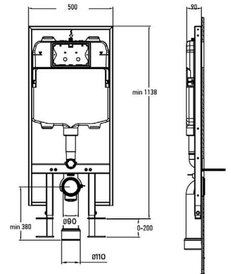
CLARICE CONCEALED TOILET TANK
