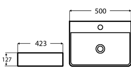
LOTUS COUNTER-TOP PORCELAIN BASIN
