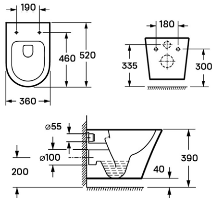
CLEMENT WALL-MOUNTED RIMLESS TOILET
