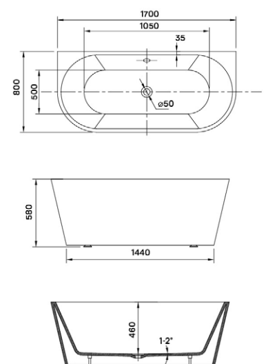
CALABRIA WHITE + CALABRIA BLACK FREESTANDING BATHTUB
