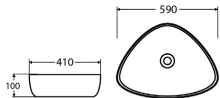
VIOLET WALL-MOUNTED PORCELAIN BASIN
