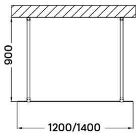
ASTRO 120/140 WALK-IN SHOWER WALL
