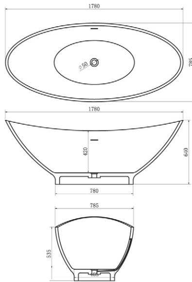
AFFAIR MATT WHITE FREESTANDING CAST MARBLE TUB
