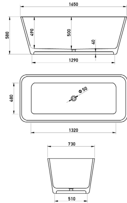
CARIB MATT WHITE + MATT BLACK FREESTANDING CAST MARBLE TUB
