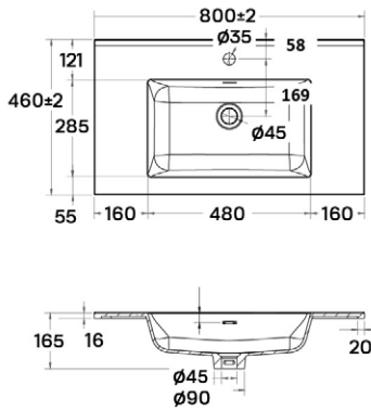
BILBAO 80 BASIN CABINET
