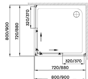
APOLLO 80/90 SHOWER CABIN
