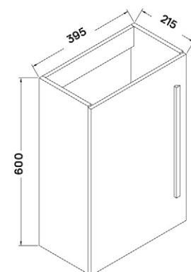
ALMERIA BASIN CABINET
