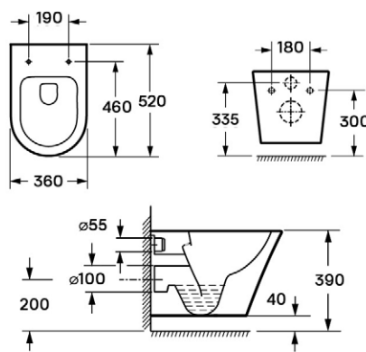
CLEMENT WALL-MOUNTED RIMLESS TOILET
