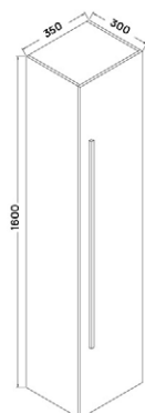
BILBAO SUSPENDED TALL CABINET
