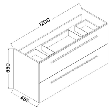
ALMERIA BASIN CABINET
